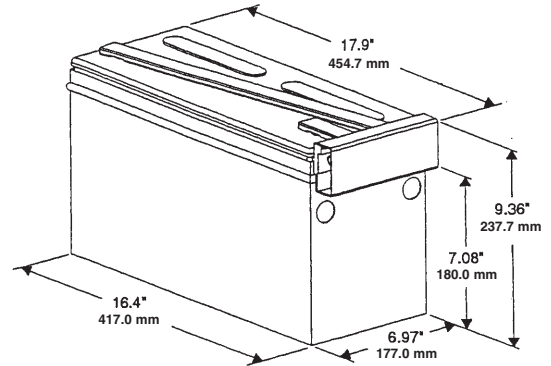
Figure 4: 12AVR-125LLP
